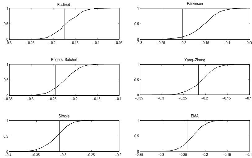
Fig. 3. Bootstrapped Values of the Maximum Likelihood GEV Shape Parameters of the Daily Volatility Weekly Maxima (Source: Euronext; 30' resampled intraday CAC40 French stock index quotes from the period 01-01-1997/12-31-2006. Computations by the authors. The bootstrapped values of the shape parameters of the Realized Volatilities are plotted on the x-axis, the empirical cumulative distribution on the y-axis).
