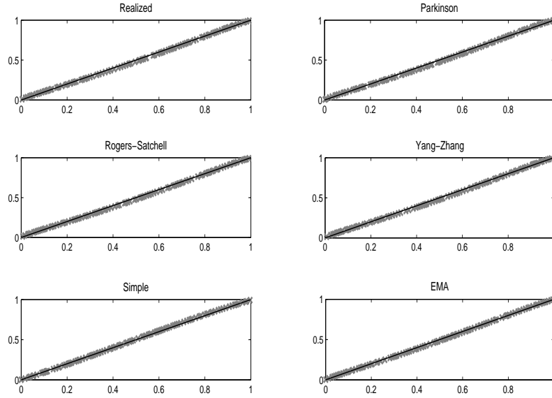
Fig. 2. Goodness-of-Fit of a Gaussian Distribution (Source: Euronext; 5' resampled intraday CAC40 French stock index quotes from the period 01-01-1997/12-31-2006. Computations by the authors. The P-P Plots show the cumulative distribution of each volatility - on the x-axis - versus the Gaussian hypothesis - on the y-axis).
