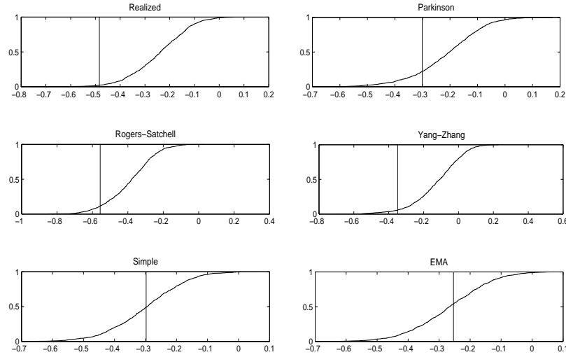
Fig. 4. Bootstrapped Values of the L-Moment method GEV Shape Parameters of the Daily Volatility Weekly Maxima (Source: Euronext; 30' resampled intraday CAC40 French stock index quotes from the period 01-01-1997/12-31-2006. Computations by the authors. The bootstrapped values of the shape parameters of the Realized Volatilities are plotted on the x-axis, the empirical cumulative distribution on the y-axis).
