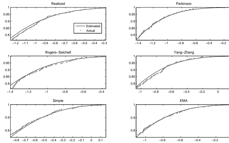
Fig. 5. Empirical and Estimated Density Functions of the Volatility Estimates (Source: Euronext; 30' resampled intraday CAC40 French stock index quotes from the period 01-01-1997/12-31-2006. Are represented in this Figure, on the y-axis, the empirical cumulative functions of the log-volatilities (dots), altogether with their GEV best fits (thin lines). Annualized Daily Volatilities are represented on the x-axis. Computations by the authors.
