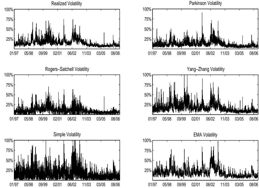
Fig. 1. Daily Estimates of Annualized Volatilities (Source: Euronext, 30' sampled intraday CAC40 French stock index quotes from the period 01-01-1997/12-31-2006. Computations by the authors).
