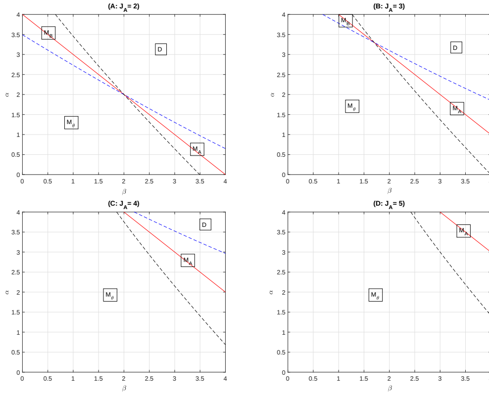
Figure 9: Monopoly/duopoly domains, for different values of J_A .
