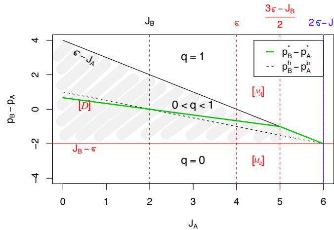
Figure 4: Phase Diagram for q under WNE, \sigma = 4 , J_B = 2 .
